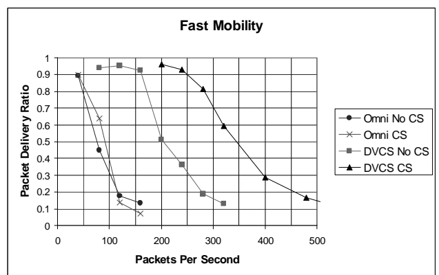
Figure 9: PDRs with and without the physical CS.
