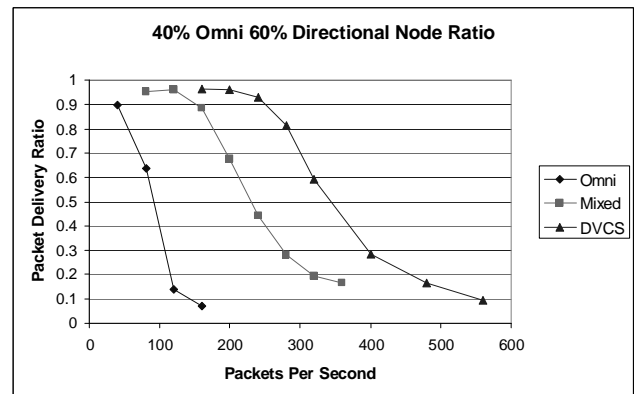
Figure 11: Mix of omni-directional and directional antennas.
