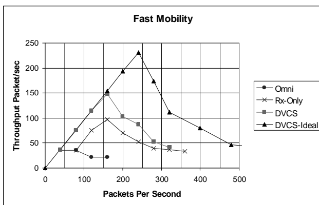
Figure 8: PDR and throughput of the network in the mobility scenario (without the physical CS in the IEEE 802.11).
