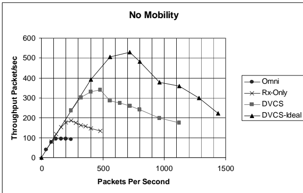
Figure 6: PDR and throughput of the network in the no mobility scenario (without the physical CS in the IEEE 802.11).
